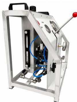
Pump side
